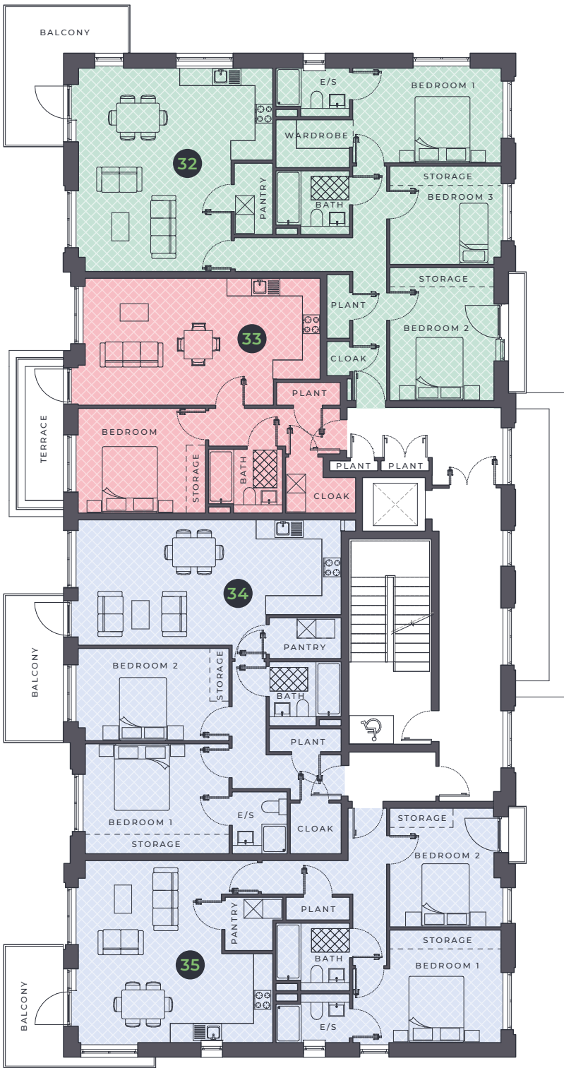
FIRST FLOOR
